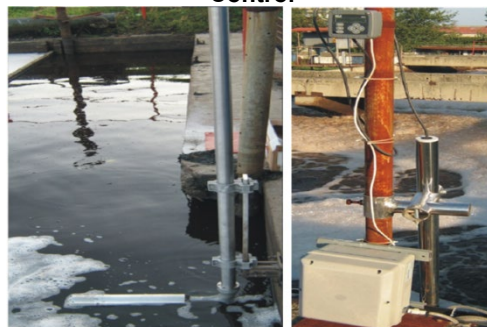
Control of the dissolved oxygen concentration in a wastewater treatment plant
